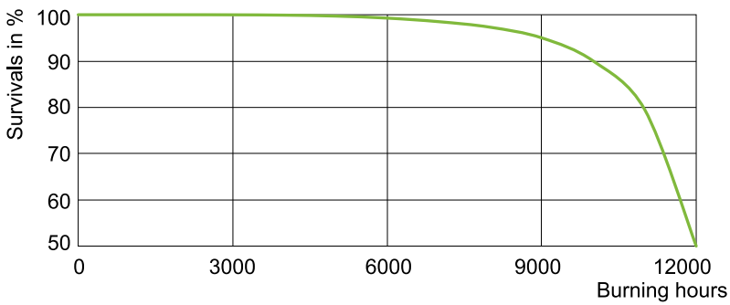
CDM-T 35W Life Expectancy /830, /842 G12
